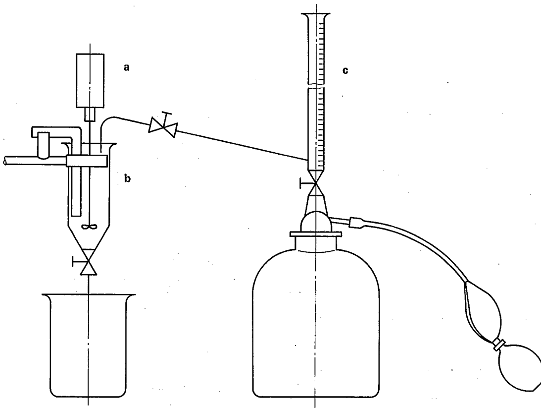
FIGURE — Special titrating apparatus
