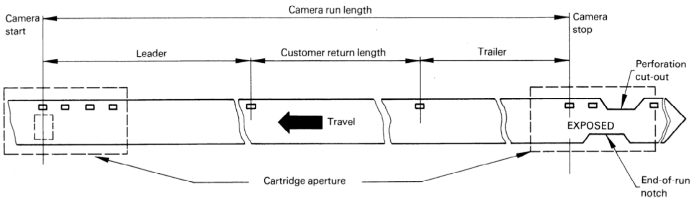
Figure 1 – Camera run length and notches
