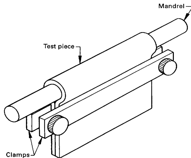
Figure 1 — Test piece holder
