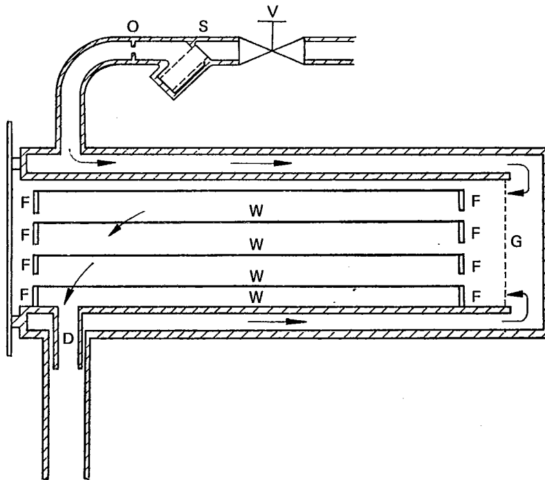
FIGURE 2 – Steaming cylinder
