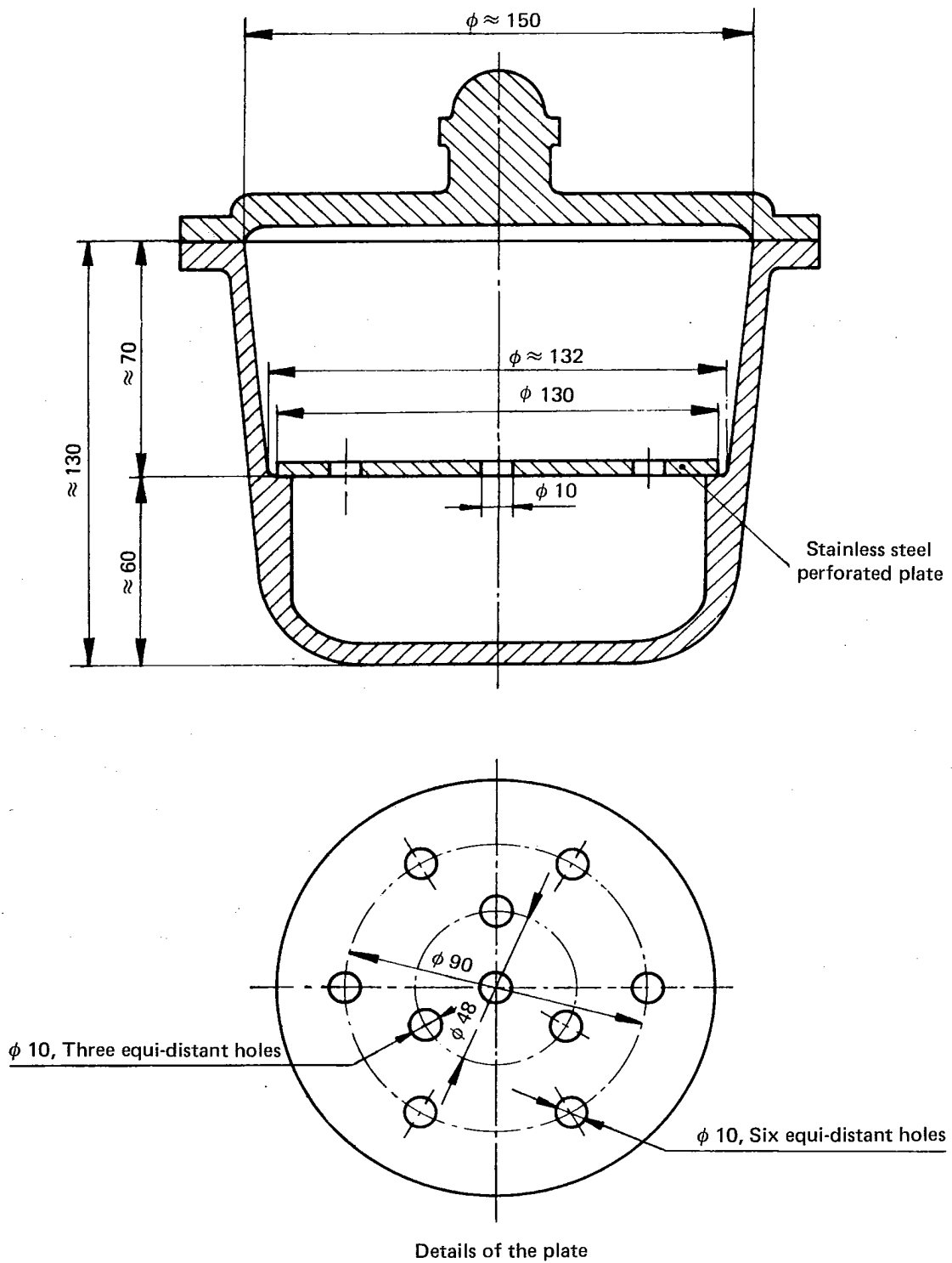
FIGURE — Glass vessel for use as a desiccator (4.2.4)
