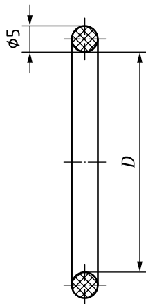
Figure 3 — O-ring
