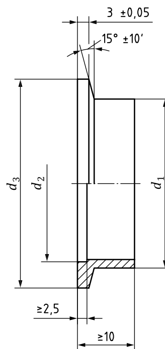
Figure 2 — Coupling
