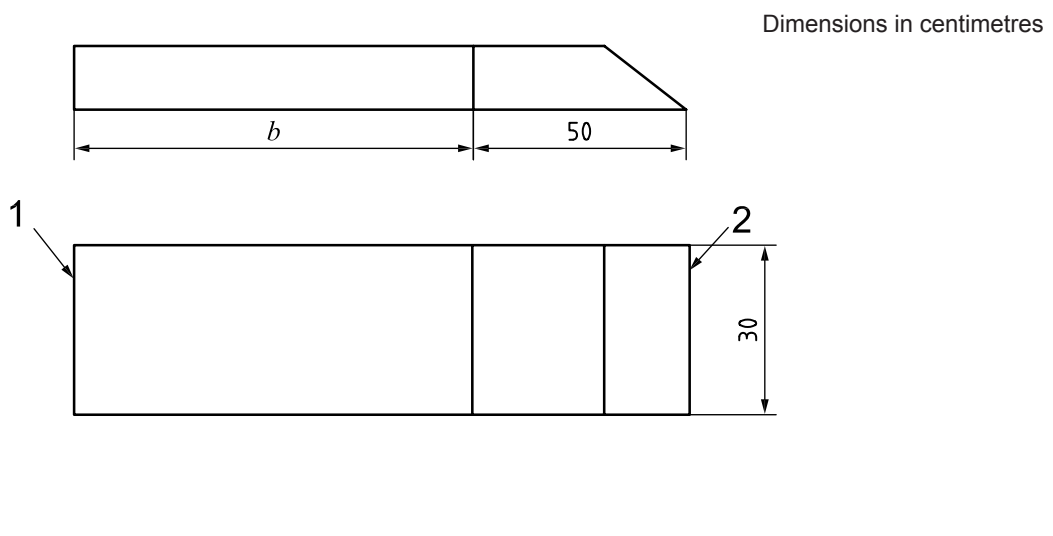
Figure A.1 — Strip cut from whole width of mat
