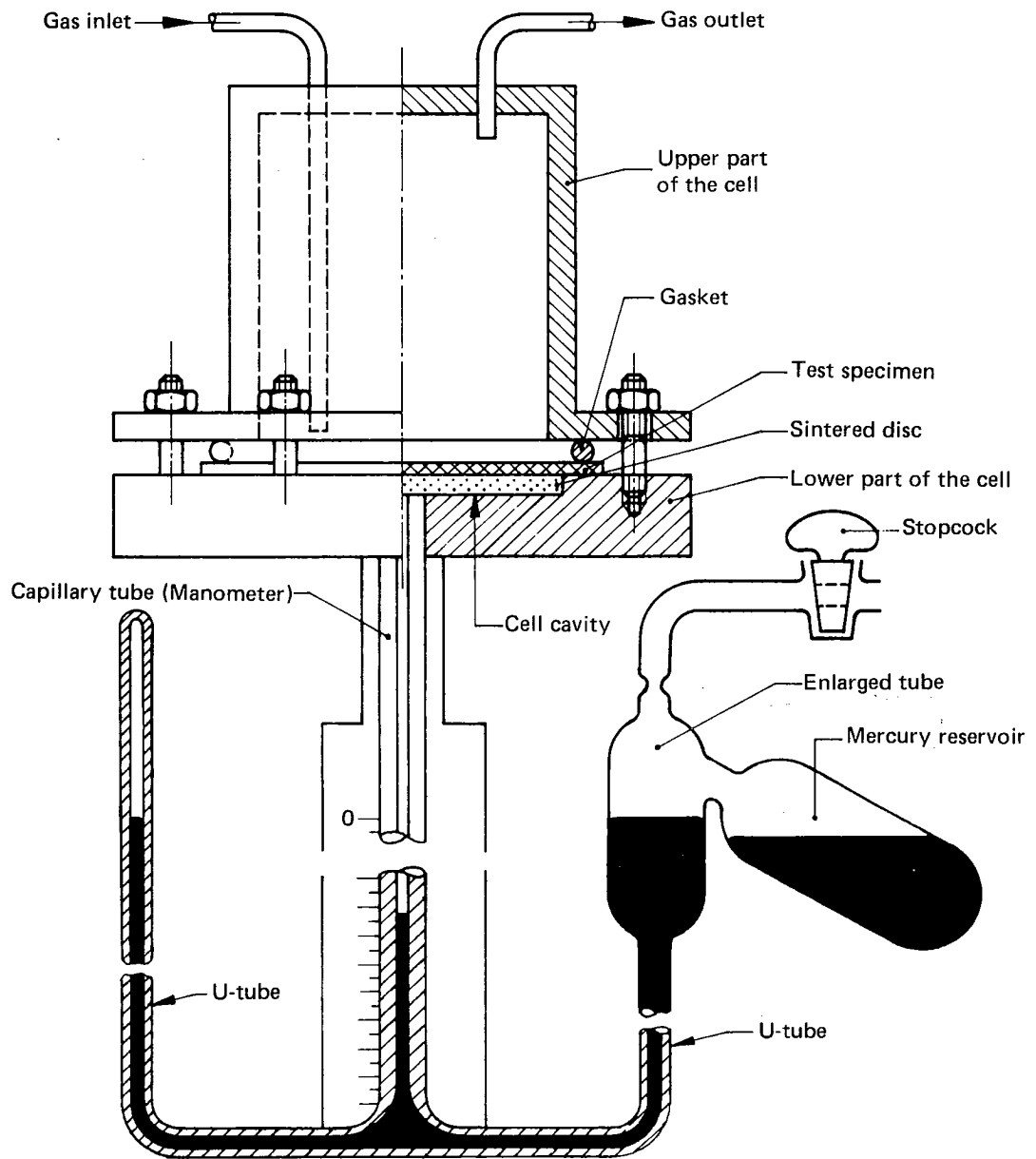
FIGURE 2 — Example of apparatus without overflowing (5.4, 2)
