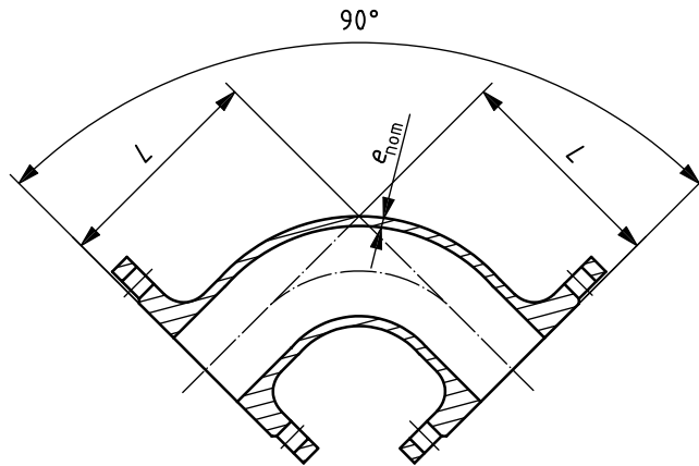
Figure 15 — Double-flanged 90° bend
