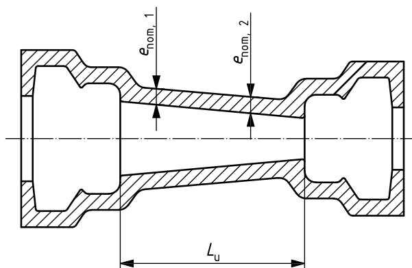
Figure 14 — Double-socket taper
