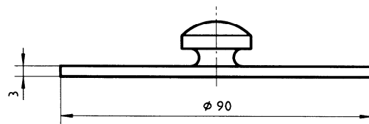
Cutting template (5.7)
