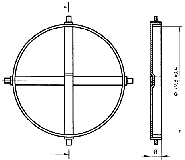
Ring template [5.3 a)]
