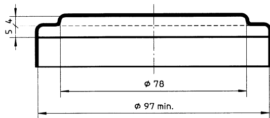
Lid (5.2) with rim to fit outside dish
