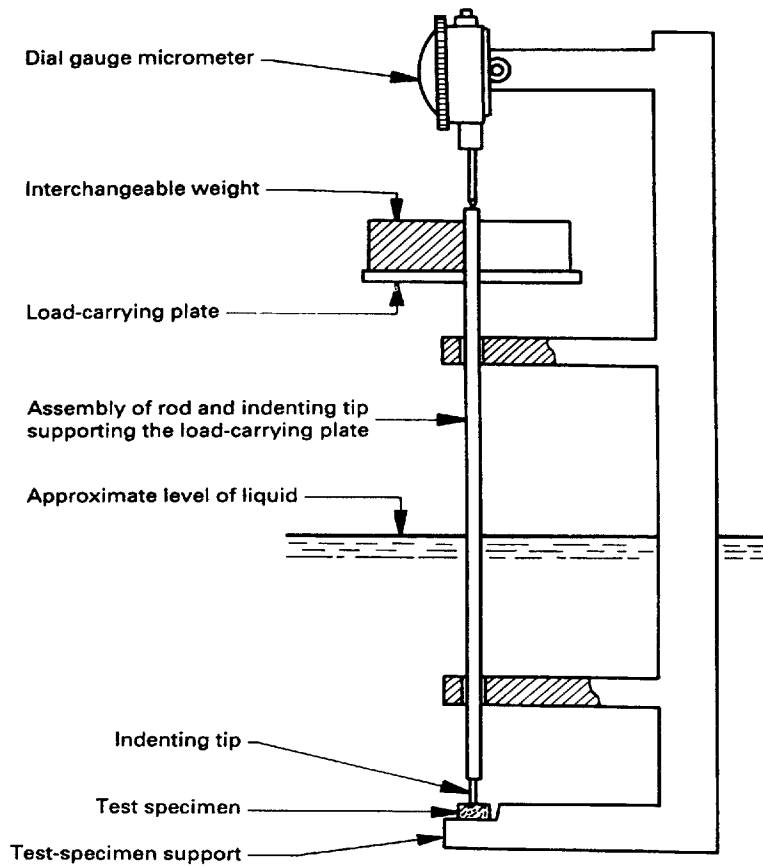
Figure 1 — Apparatus for determining the Vicat softening temperature
