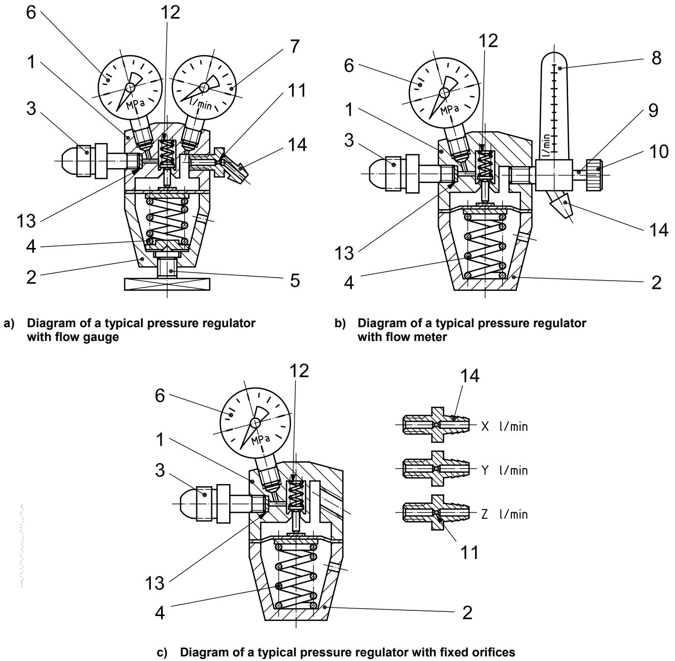
Figure A.2 — Typical pressure regulators
