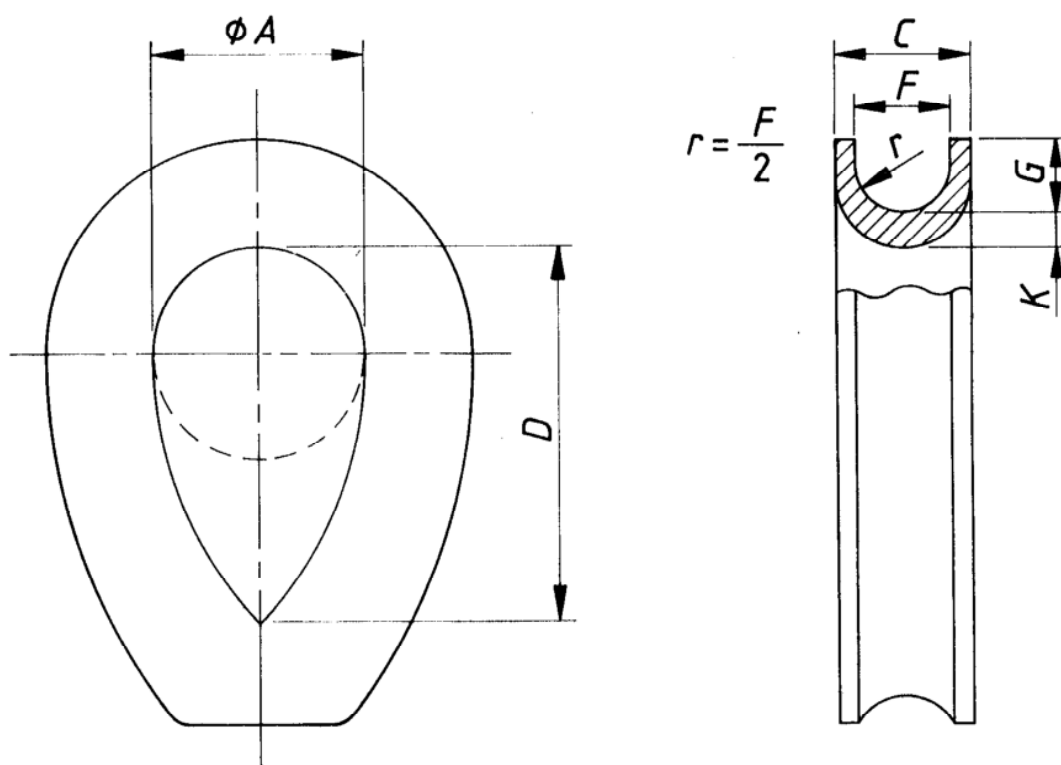
Figure 2 — Thimble without point
