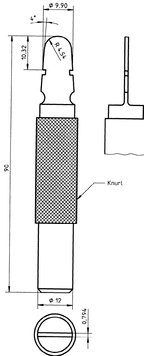
Figure 3 — Cup plug gauge
