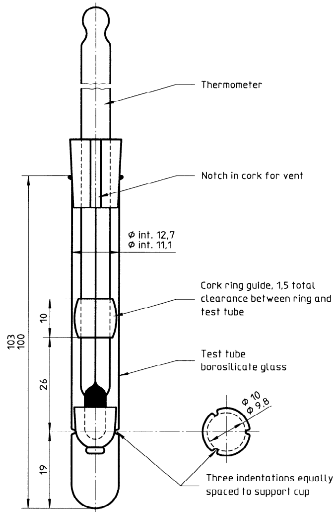
Figure 2 — Assembled apparatus
