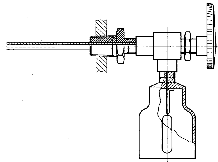
Figure 8 — Needle sampler
