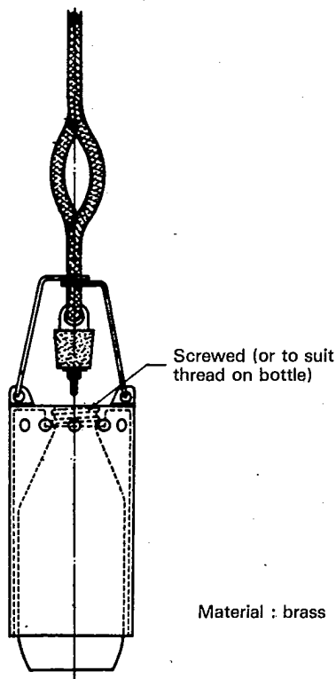
Figure 2 — Example of sampling cage for use with screw-top glass 600 ml sample bottle
