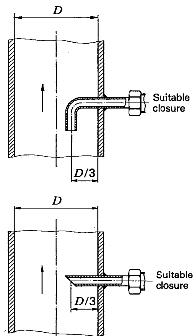
Figure 7 — Typical pipeline sampling apparatus
