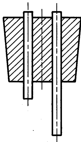
Figure 6 — Stopper for representative sampling
