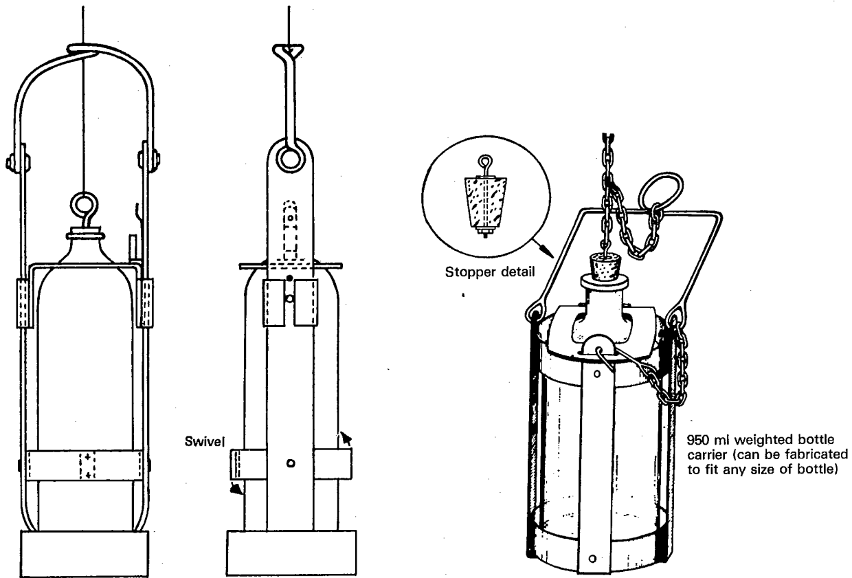
Figure 1 — Examples of sample cages
