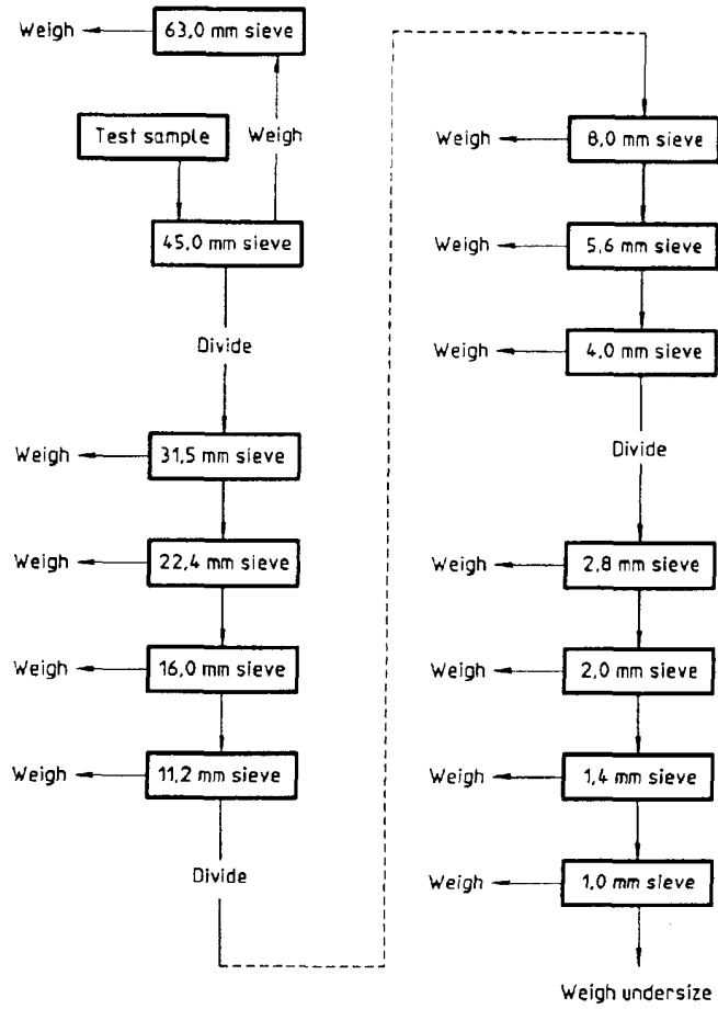
Figure 1 — Schematic diagram of a sieving procedure
