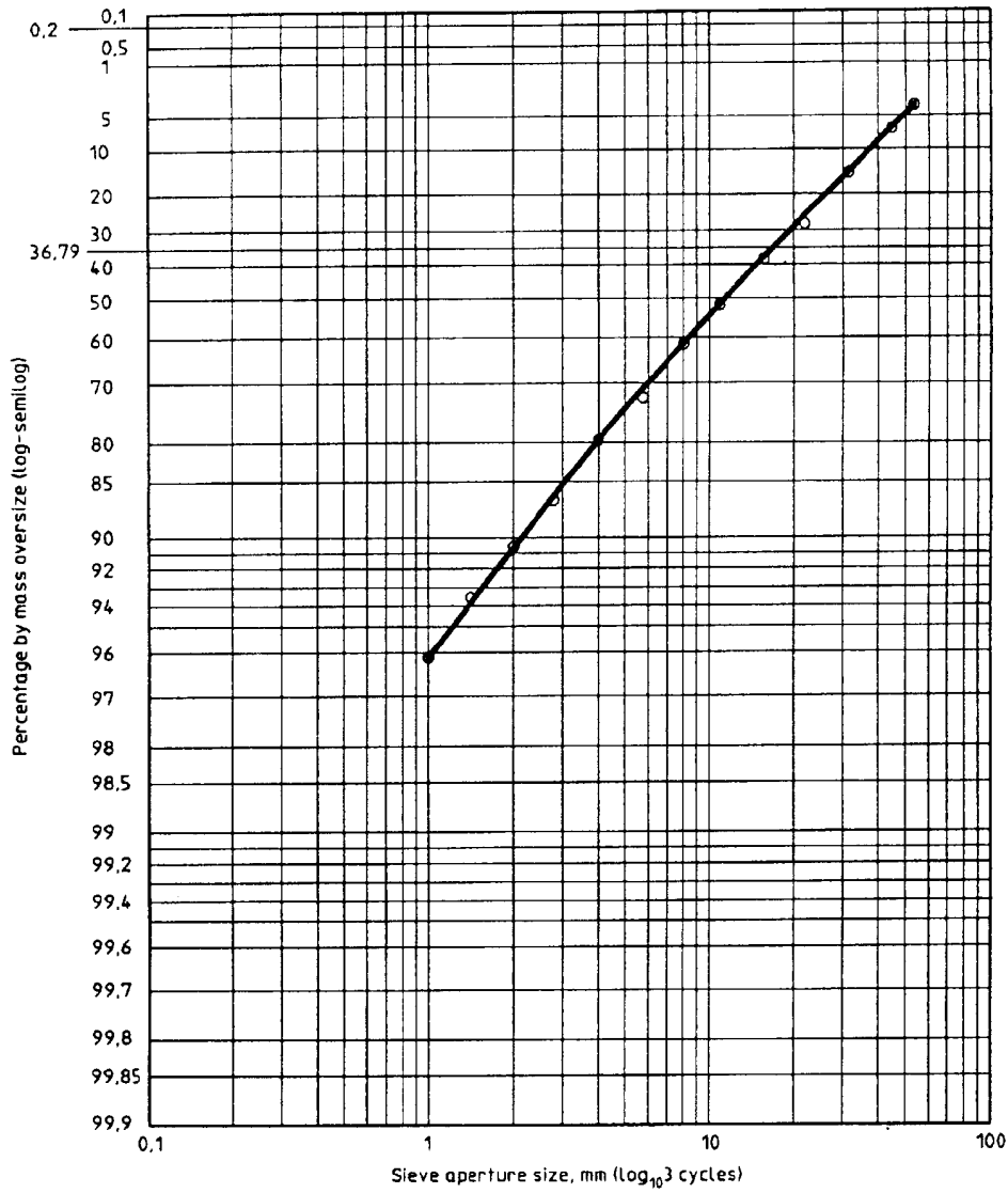
Figure 2 — Graphical presentation of a size analysis
