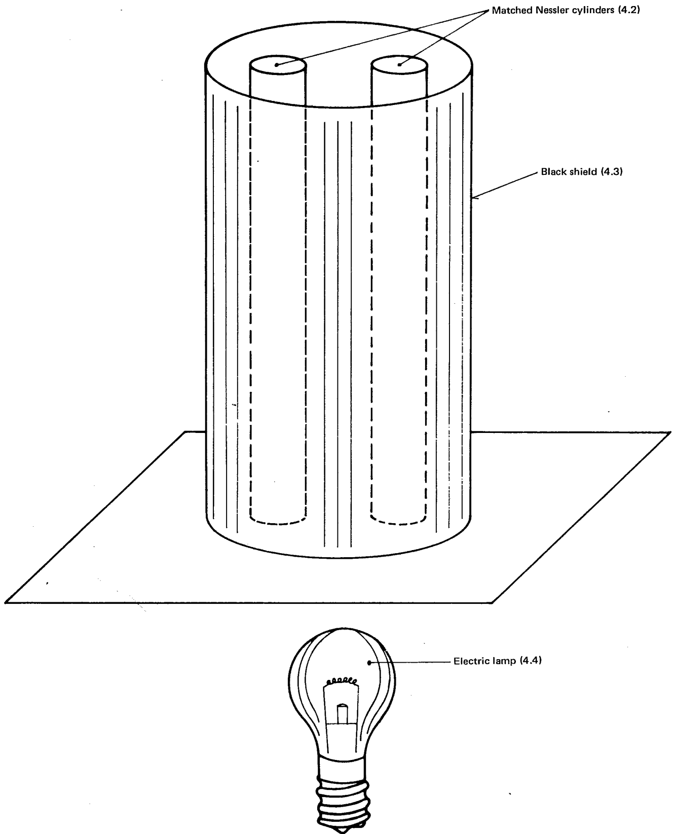
FIGURE — Apparatus for use in the visual test for impurities insoluble in water
