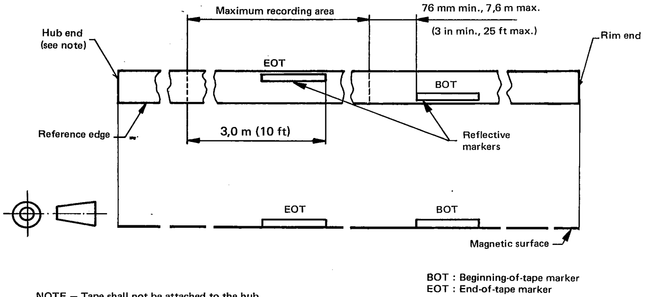
FIGURE 3 — Reflective markers and recording area
