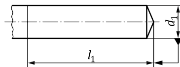
Figure 2 — Type 2 and Type 4 shank
