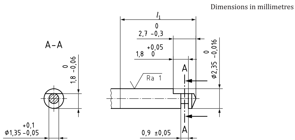
Figure 4 — Dimensions Type 1 shank
