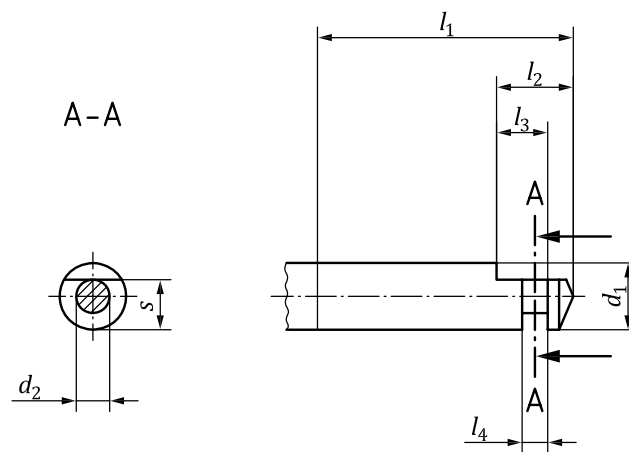
Figure 1 — Type 1 shank
