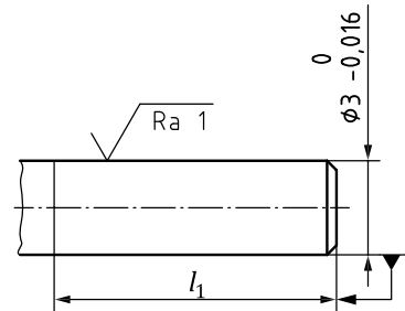
Figure 7 — Dimensions Type 4 shank
