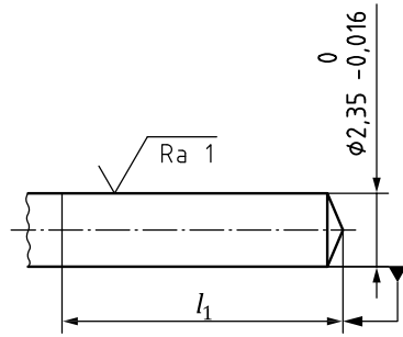
Figure 5 — Dimensions Type 2 shank
