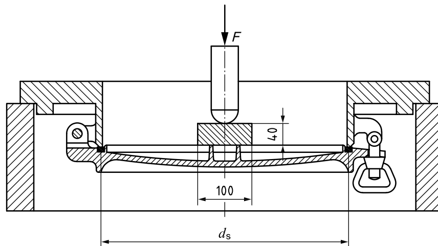
Figure 6 — Prototype test
