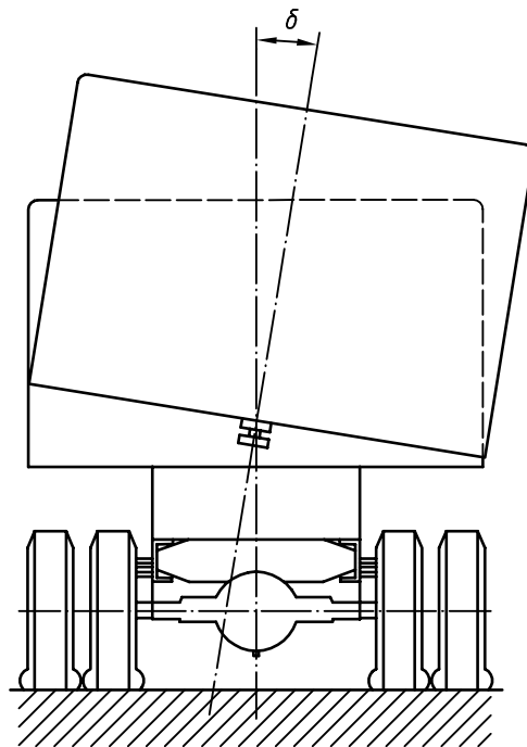
Figure 4 — Lateral inclination
