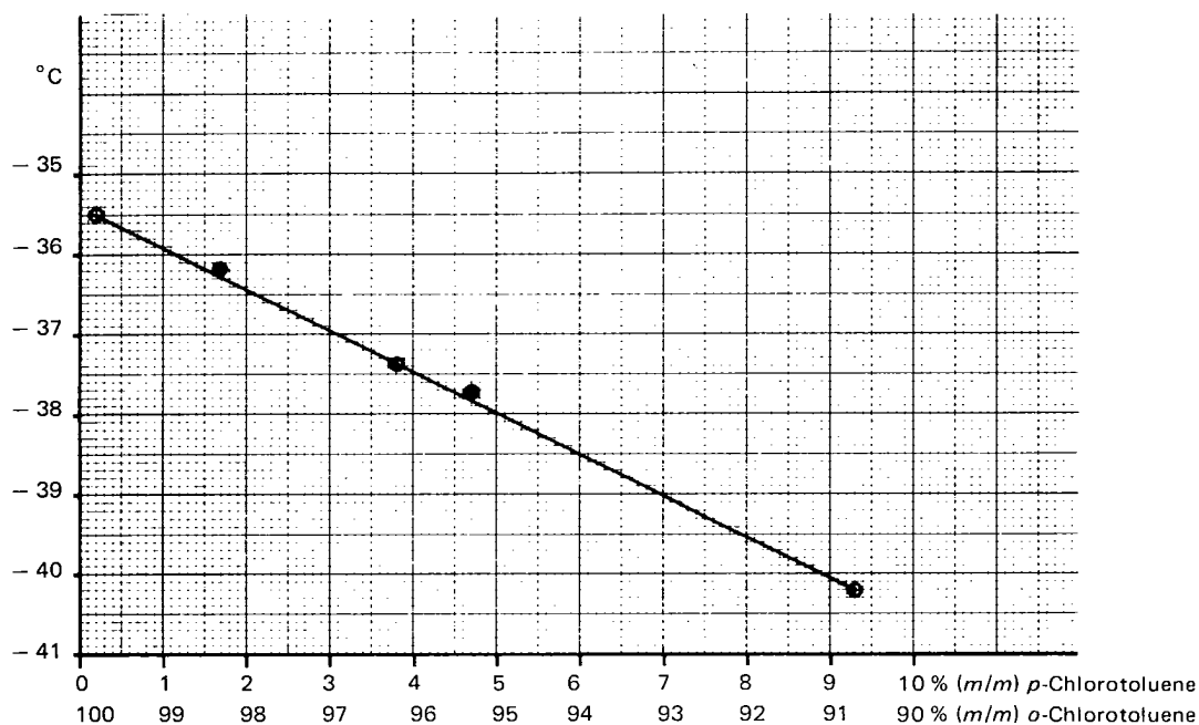
FIGURE 2 – Crystallizing point diagram of the o-p -chlorotoluene system, for the range 0 to 9 % (m/m) p -chlorotoluene
