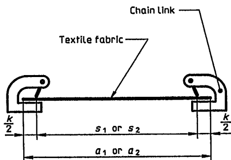
Figure 2 — Machines and plant with tenting chains
