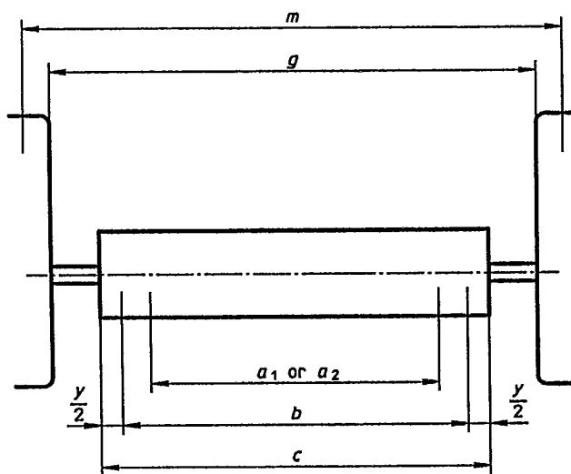
Figure 1 — Machines and plant — General plan
