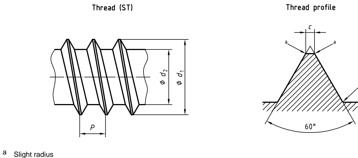
Figure 1 — Thread dimensions
