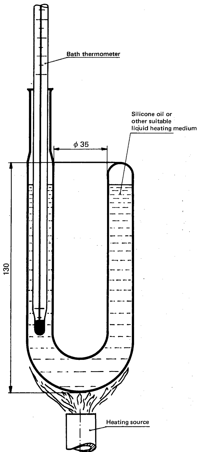
FIGURE 4 – Heating bath
