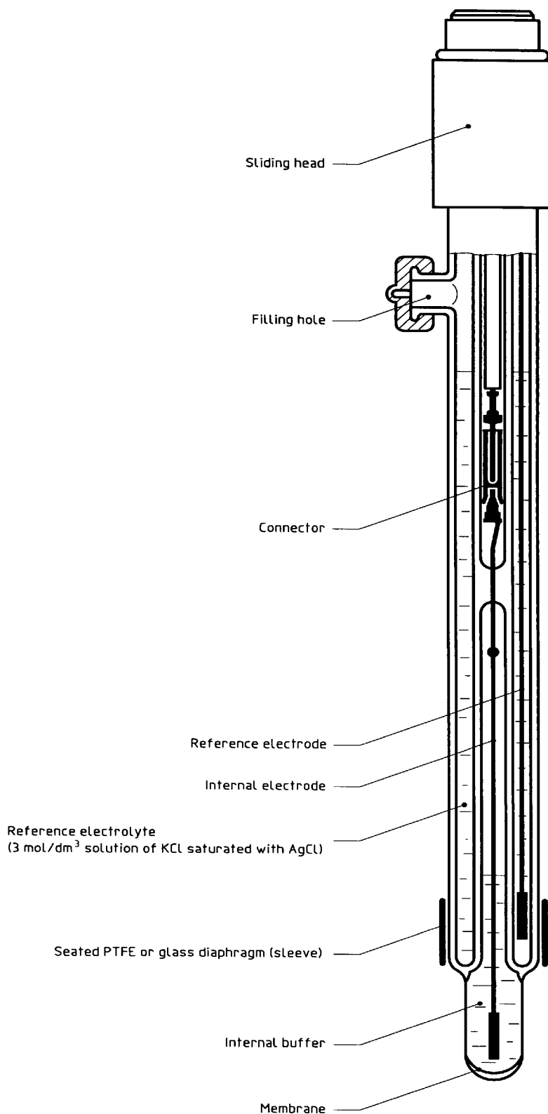
Figure 1 — Typical combined electrode
