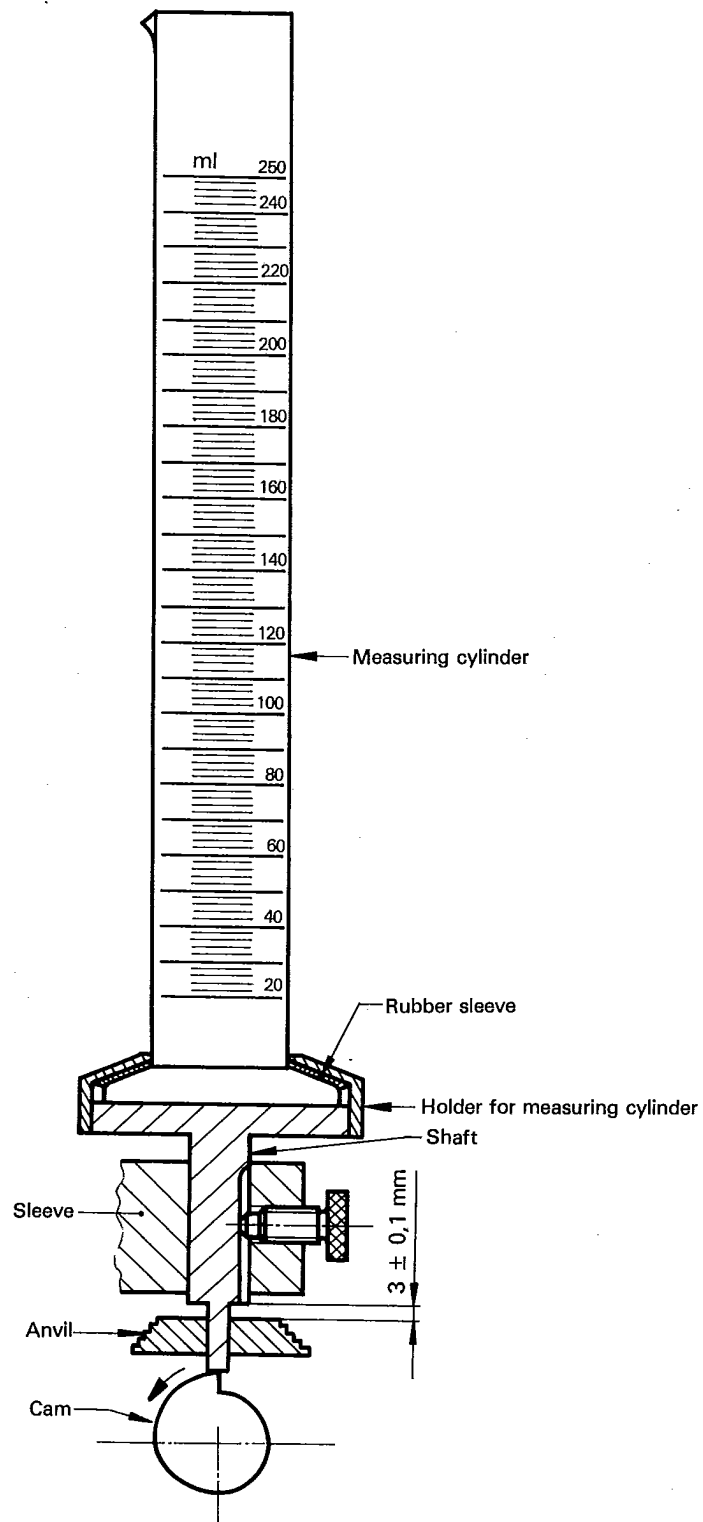
Figure — Tamping volumeter
