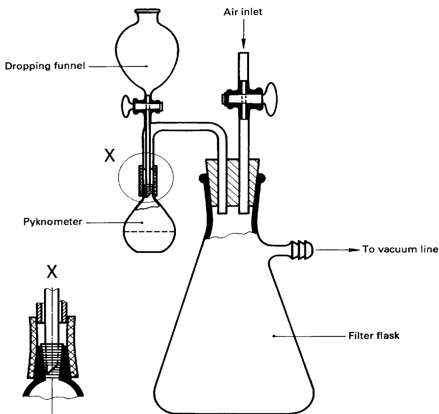
Figure 2 — Vacuum apparatus
