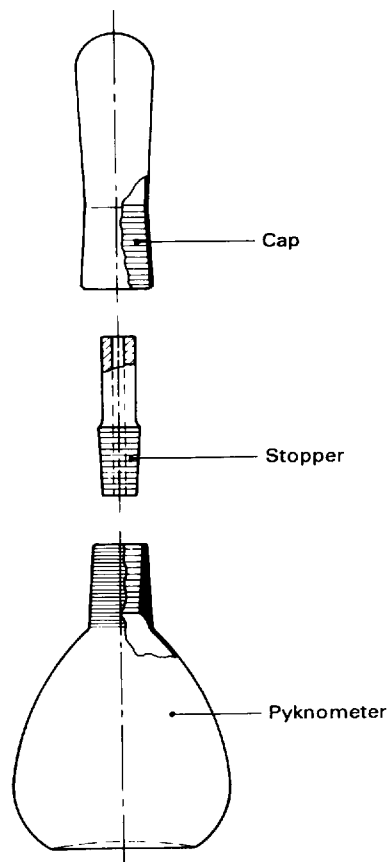
Figure 1 — Pyknometer, Gay-Lussac type
