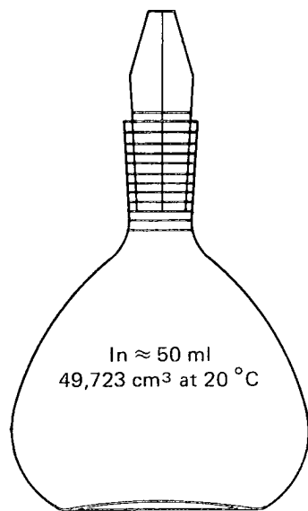
FIGURE — 50 ml pycnometer flask, type 3 (Gay-Lussac)
