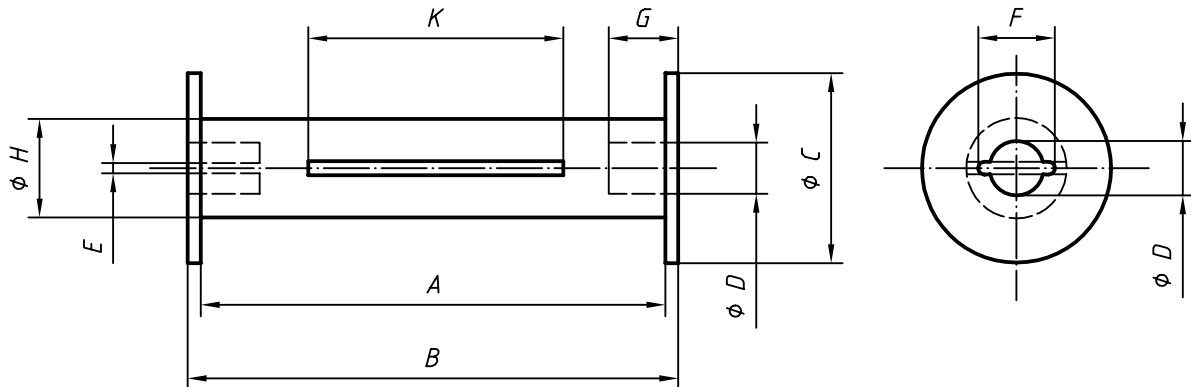
Figure 3 — Spool dimensions
