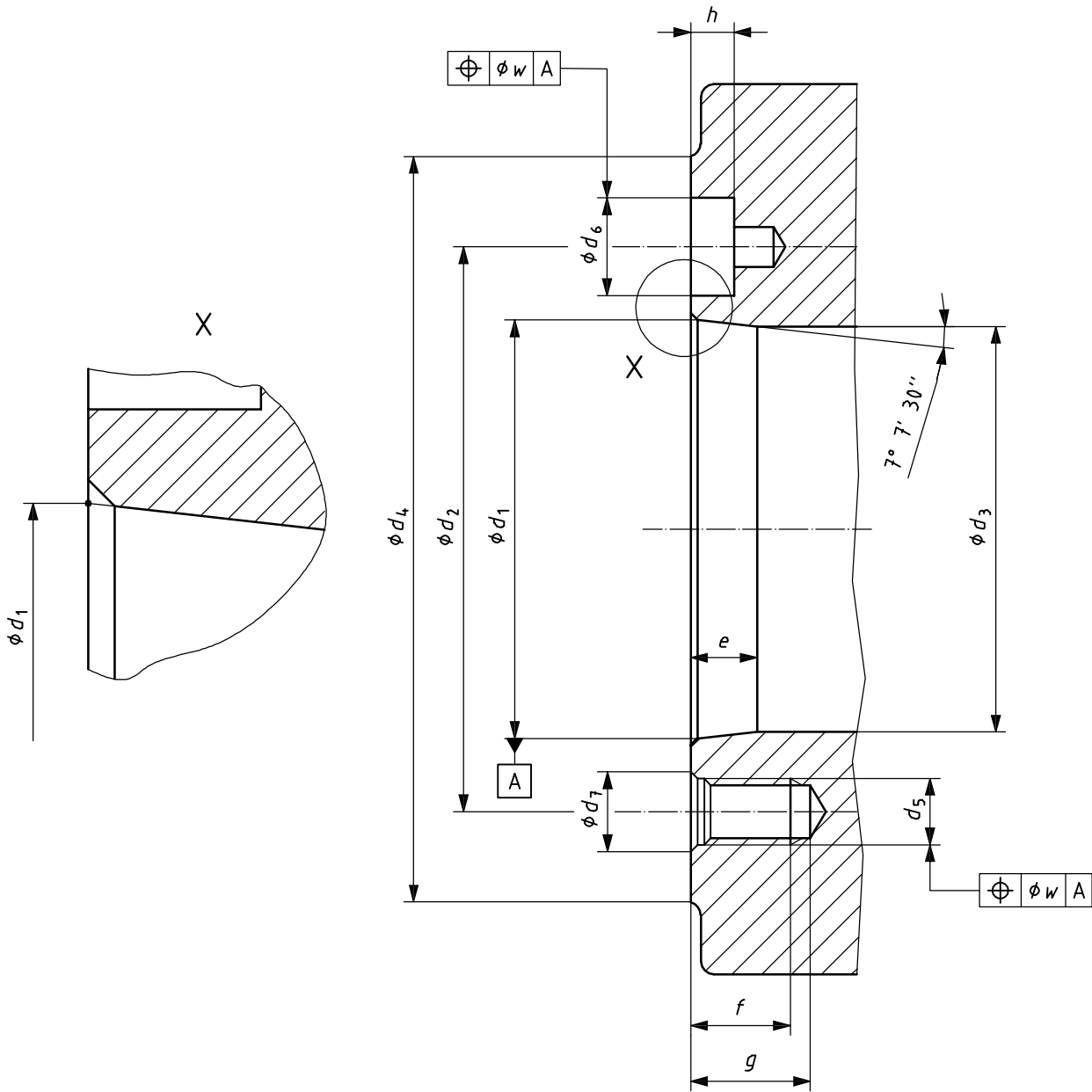
Figure 3 — Face plates
