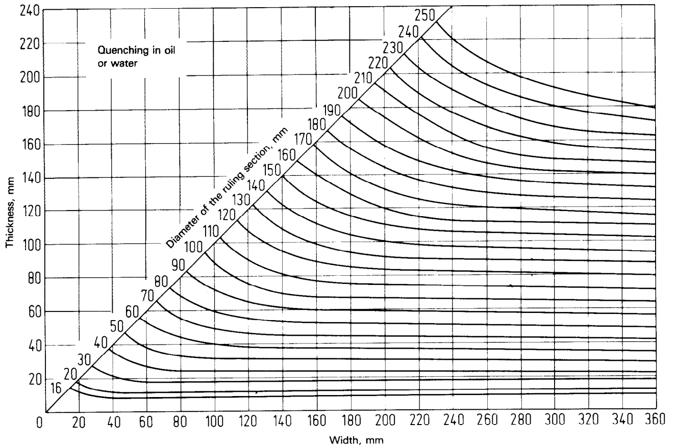
Figure 2 — Diameter of the ruling section of square and rectangular bars
