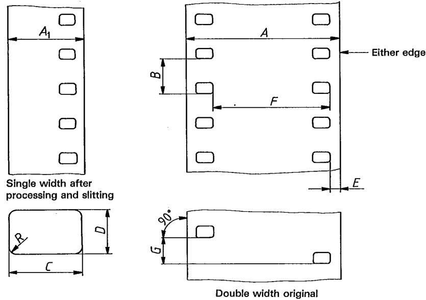
Figure — 16 mm film perforated 8 mm Type R
