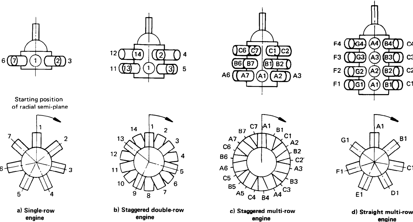
FIGURE 4 – Numbering of cylinders of radial piston engines
