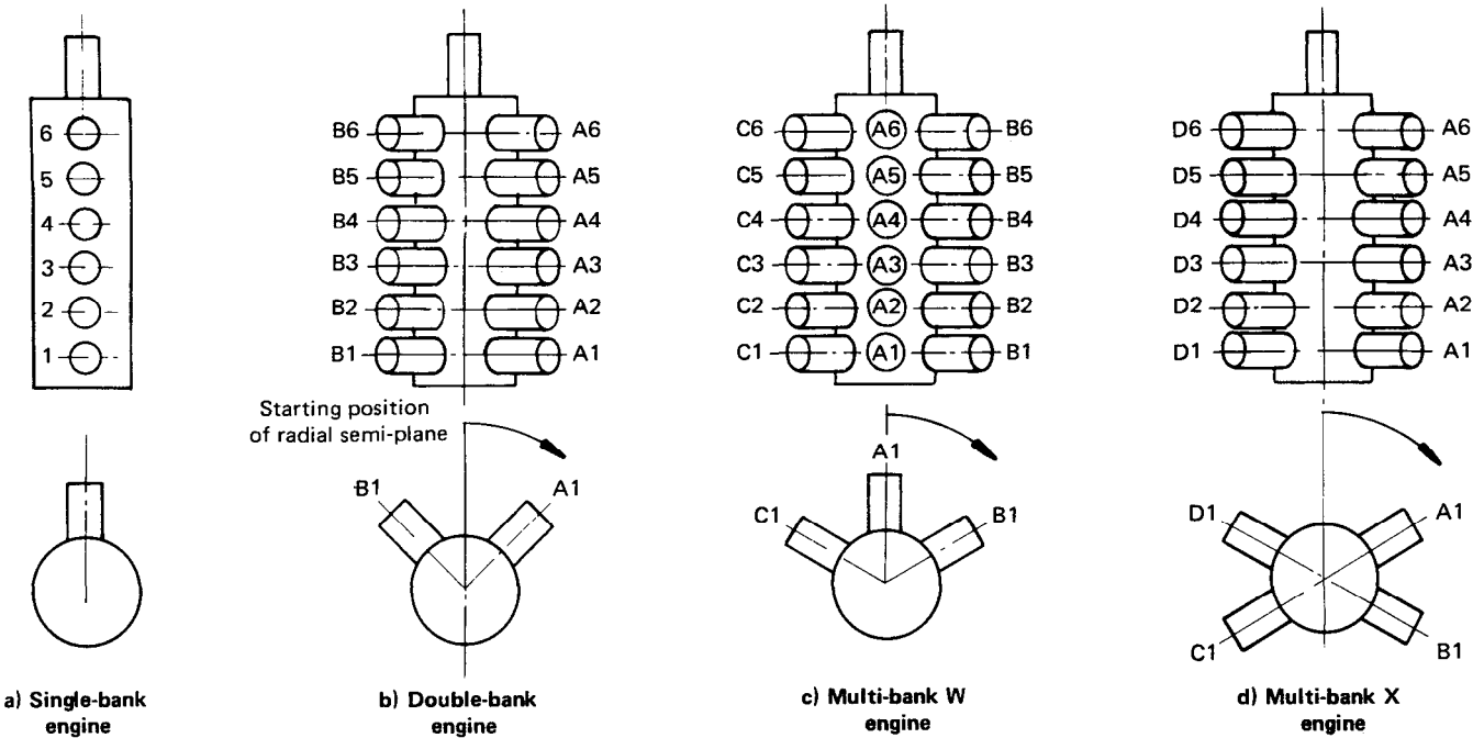
FIGURE 3 – Numbering of cylinders of in-line piston engines
