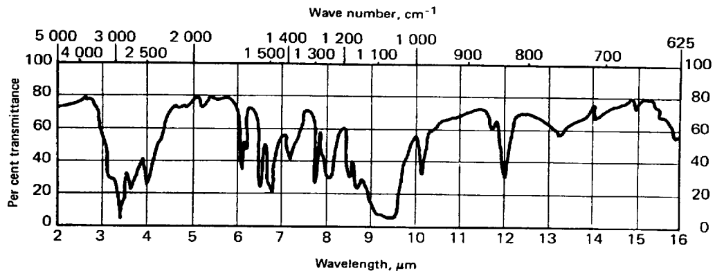
Figure 1 — Reference infrared spectrum of p -methylaminophenol sulfate (KBr plate)
