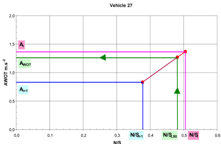
Figure A.16 — Determination of wide-open-throttle acceleration a_{wot\ 50}
