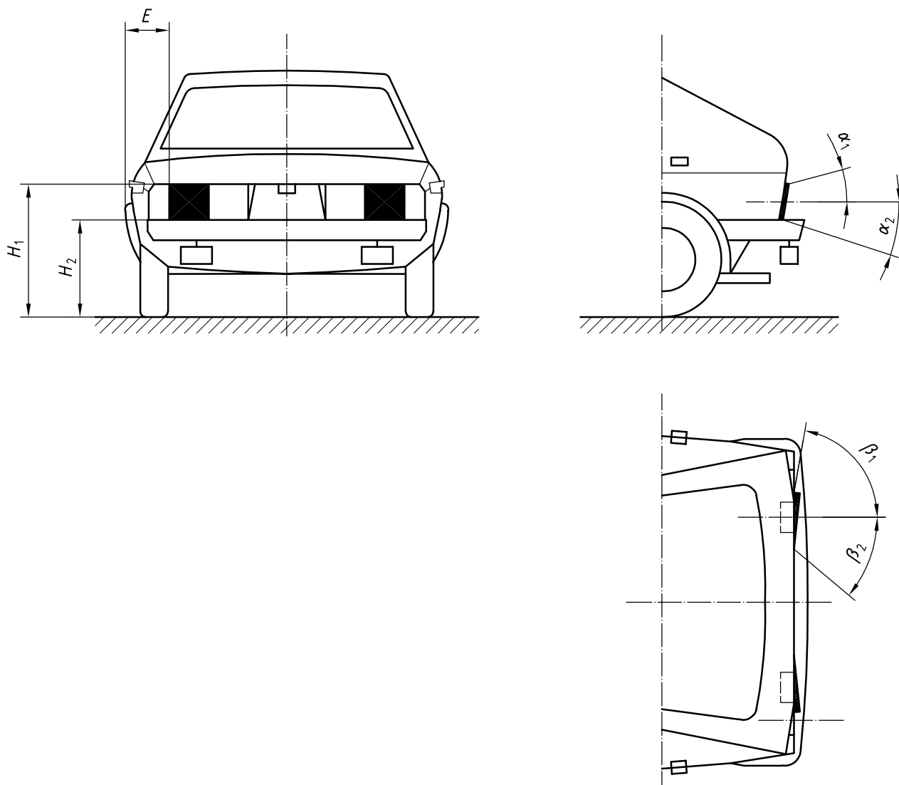
Figure E.12 — Rear position lamp
