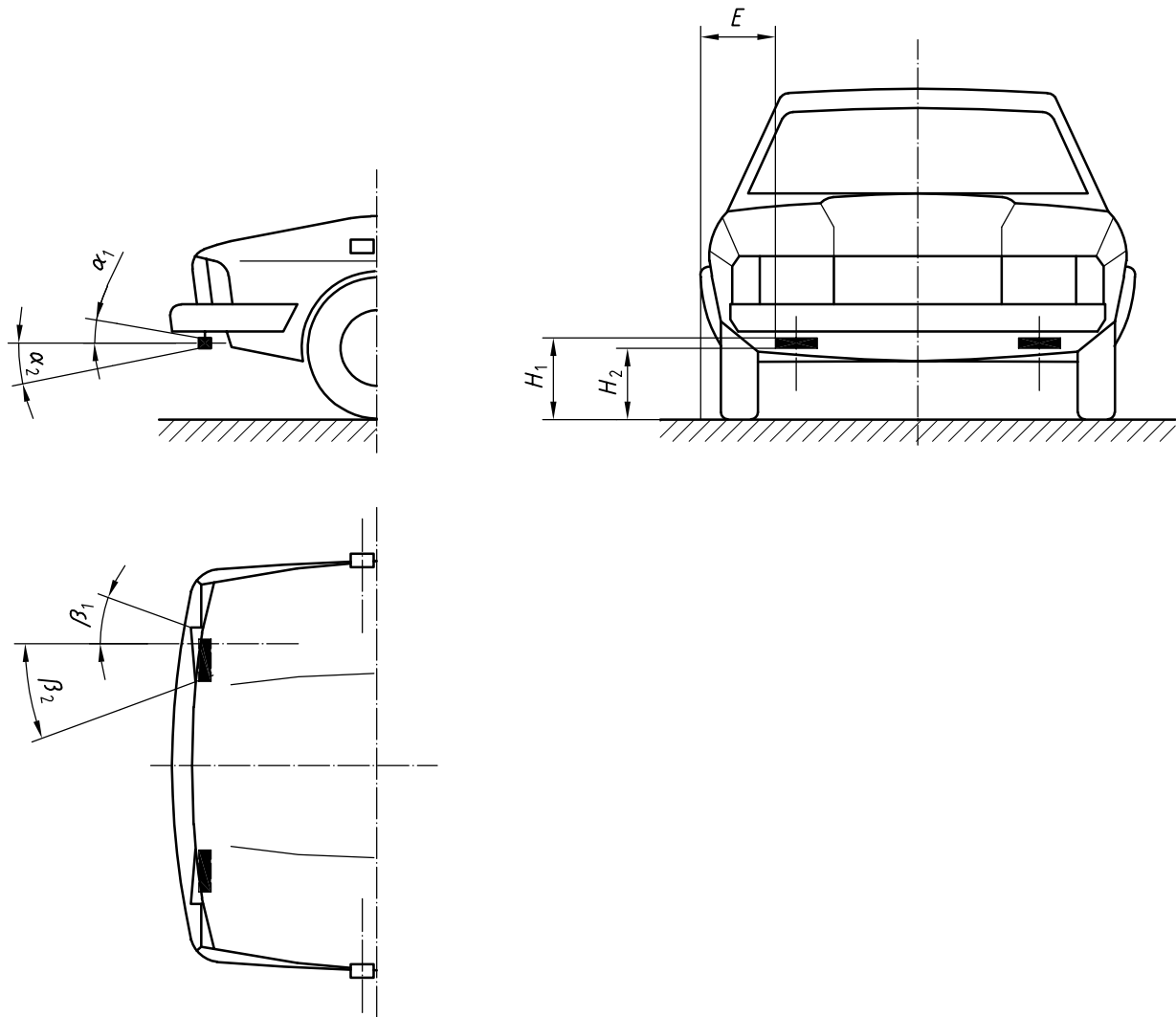
Figure E.25 — Daytime running lamp
