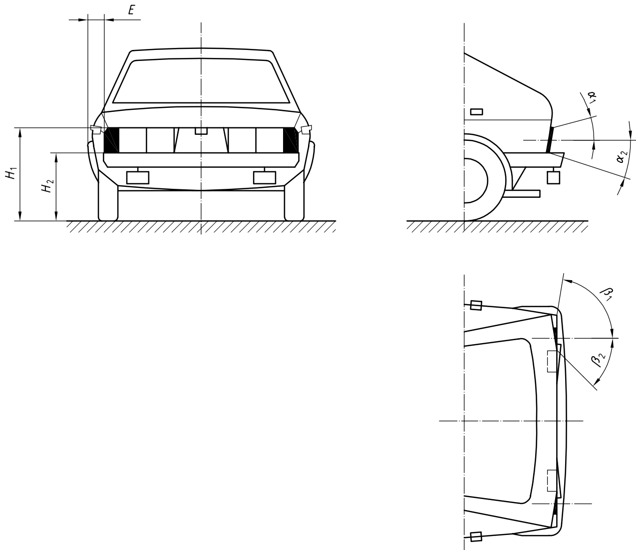
Figure E.9 — Rear direction indicator lamp
