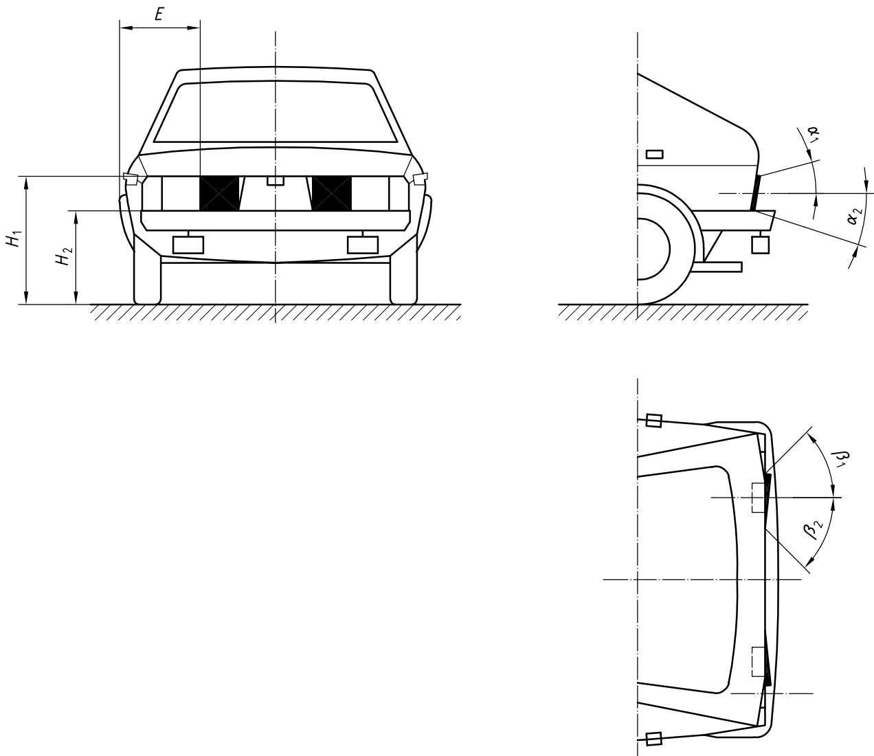
Figure E.10 — Stop lamp
