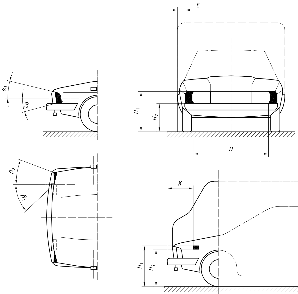
Figure E.26 — Cornering lamp
