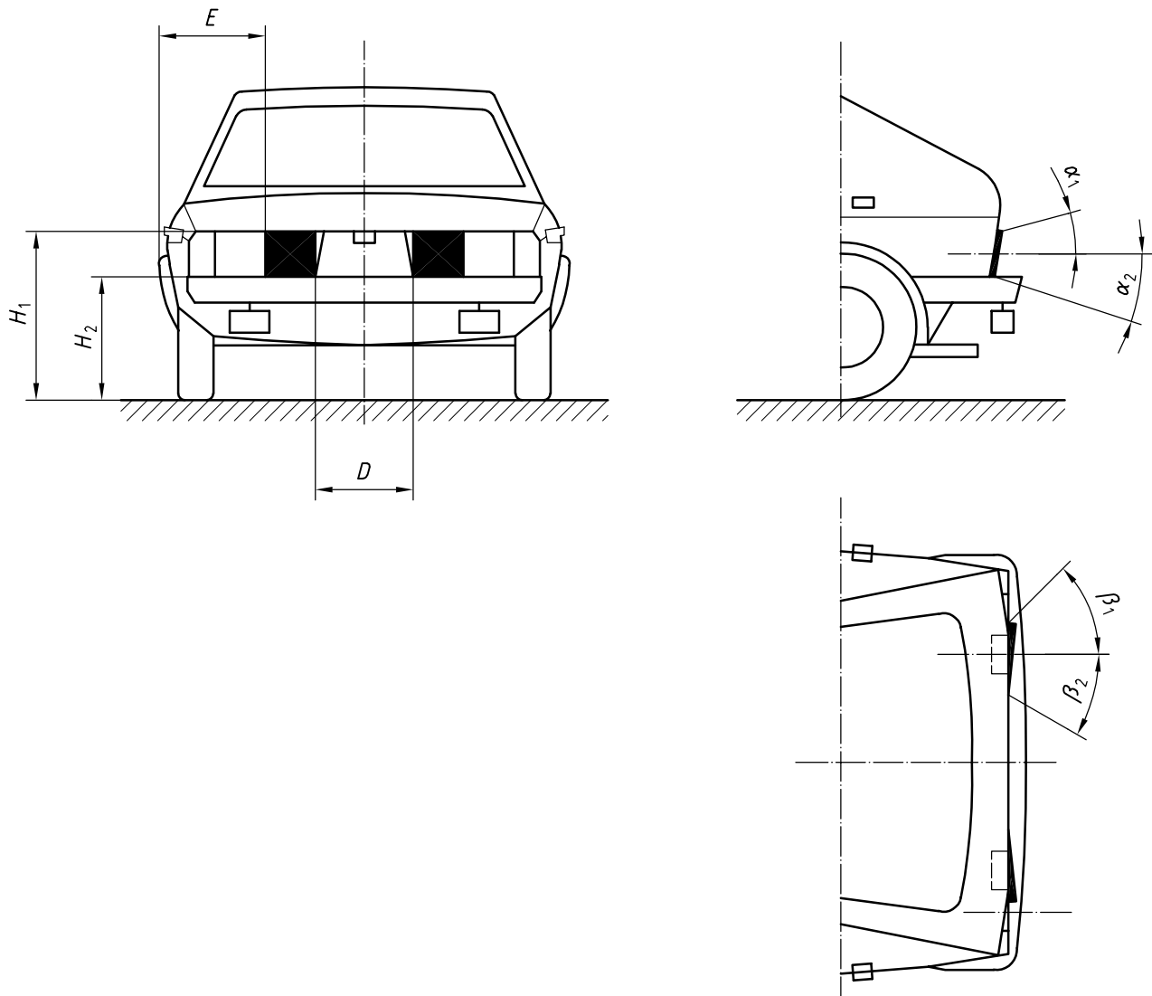
Figure E.14 — Reversing lamp
