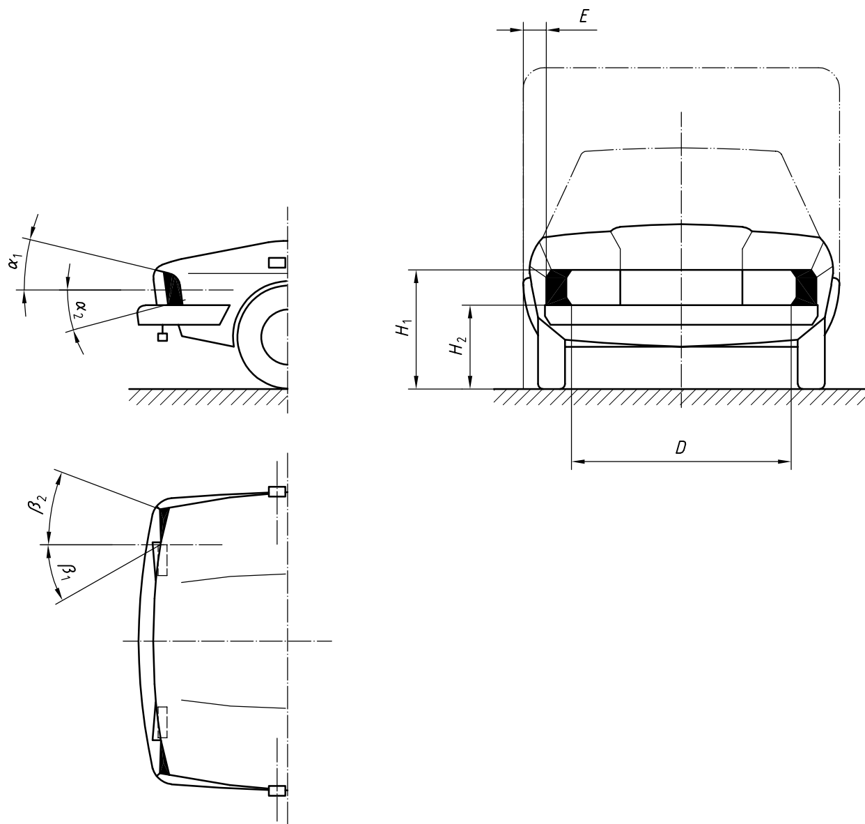
Figure E.23 — Front, non-triangular, retro-reflector
