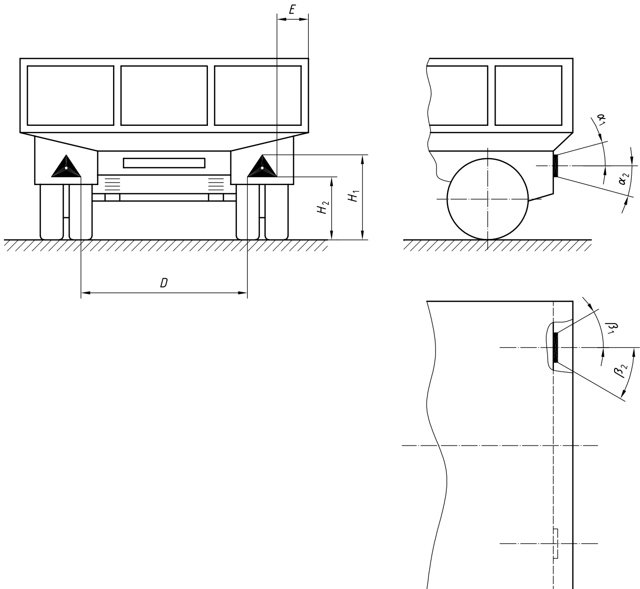
Figure E.24 — Rear triangular retro-reflector
