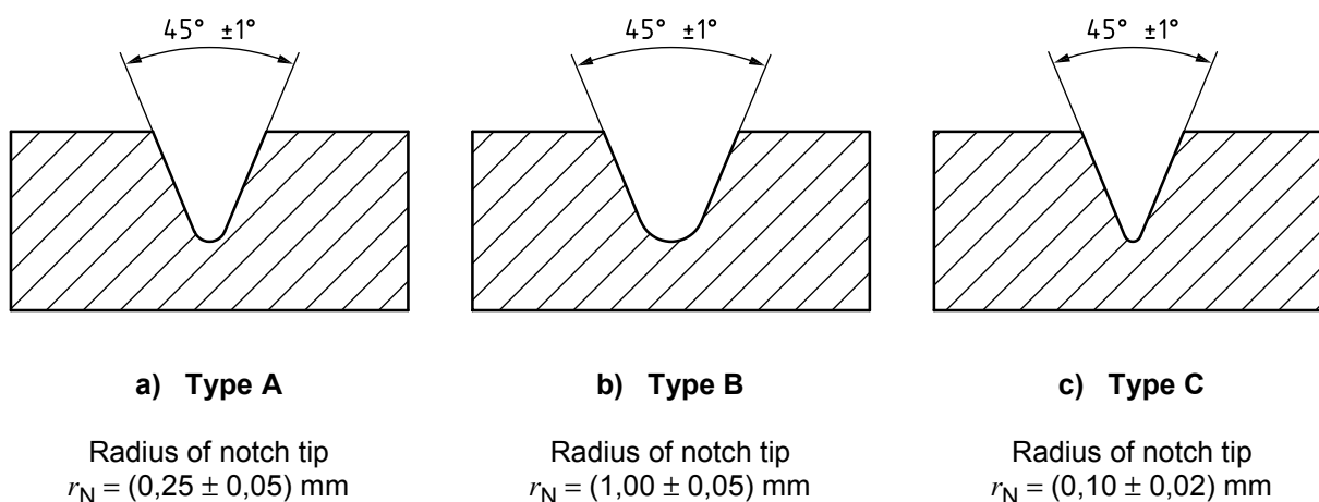
Figure 5 — Notch types
