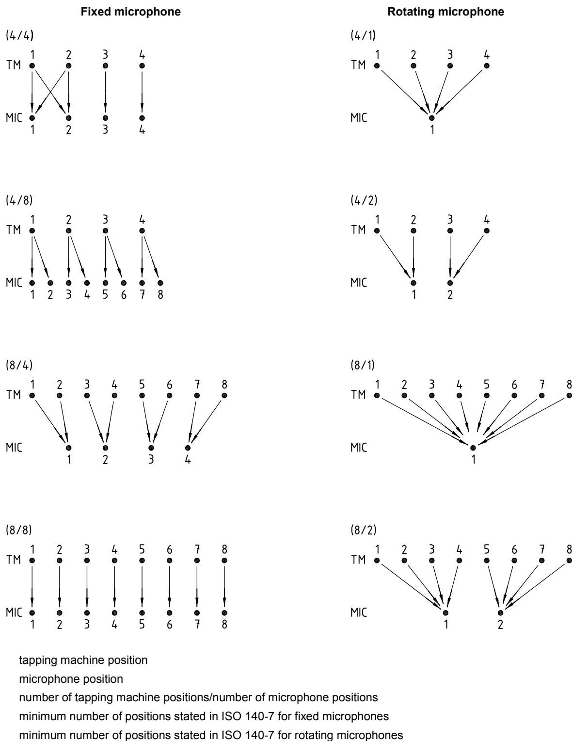
Figure D.1 — Examples of positions of tapping machines and microphones
