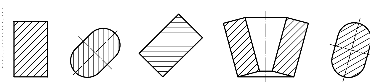
Figure 1 — Hatching of areas of cuts or sections — Examples
