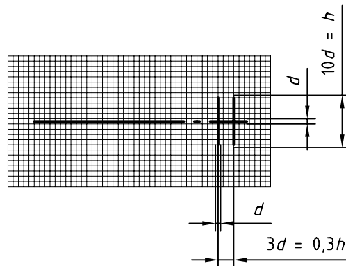
Figure C.3 — Graphical symbol for symmetry
