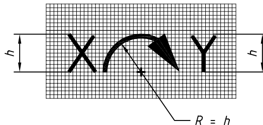
Figure C.2 — Graphical symbol for arc arrows
