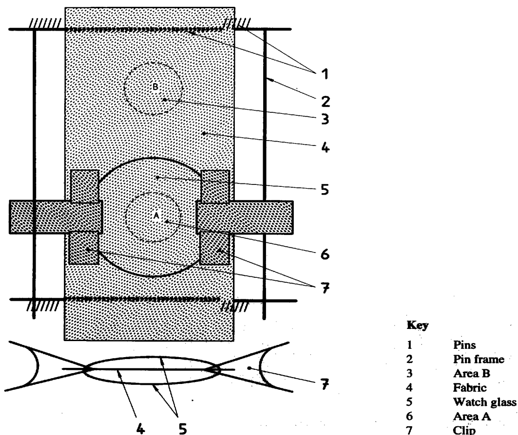
Figure 2 — Layout of apparatus for inducing colorant migration using procedure B
