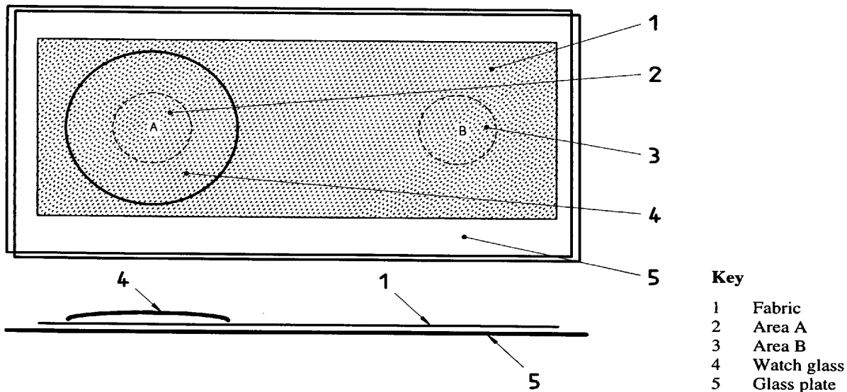
Figure 1 — Layout of apparatus for inducing colorant migration using procedure A
