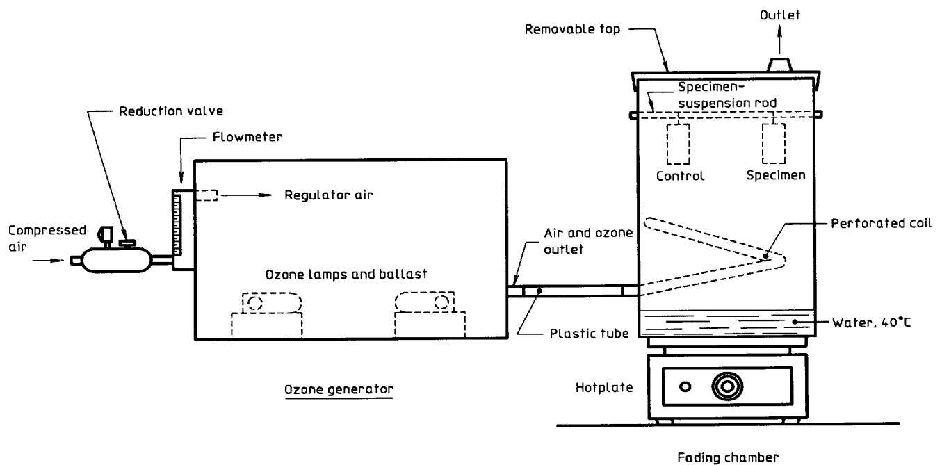
Figure A.1 — Typical test arrangement
