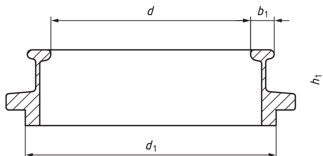
Figure 1 — Example of a T-ring
