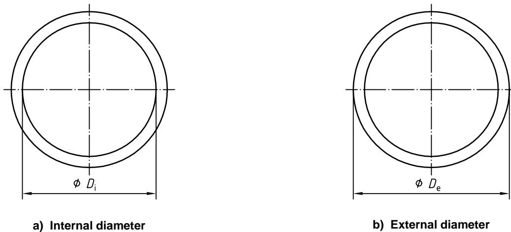
Figure 7 — Diameters
