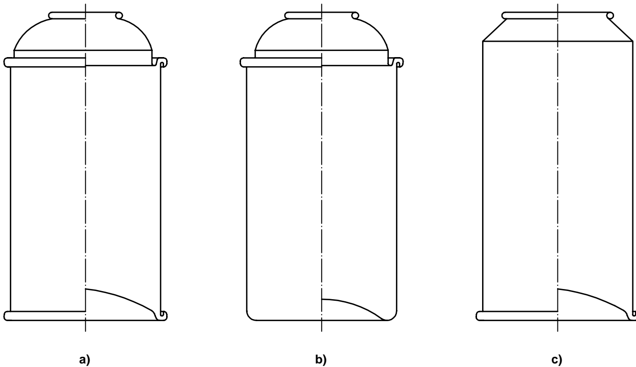
Figure 5 — Straight-sided can
