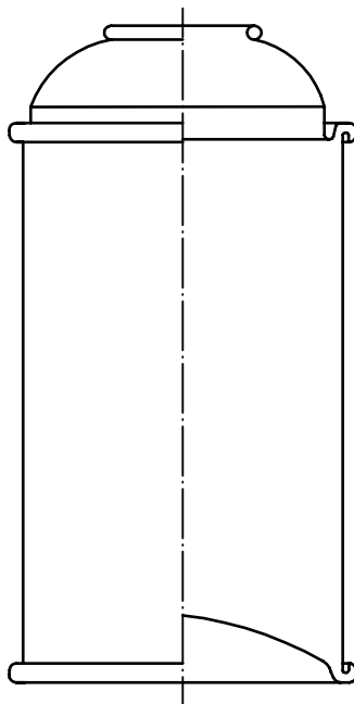
Figure 2 — Three-piece can
