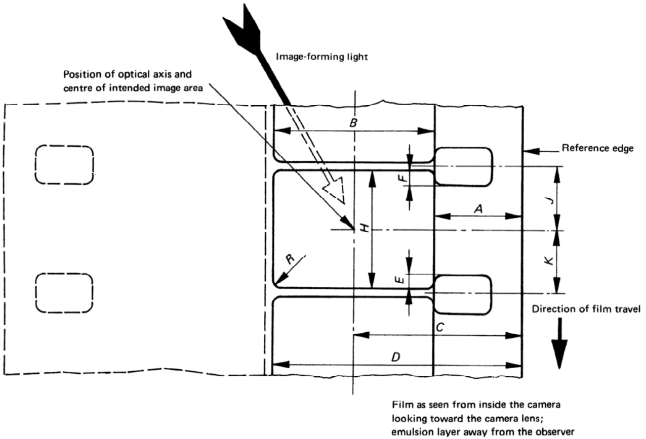
FIGURE 1 – Image area produced by camera aperture
