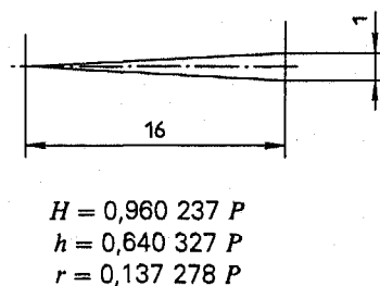
Figure 2 — Taper thread
