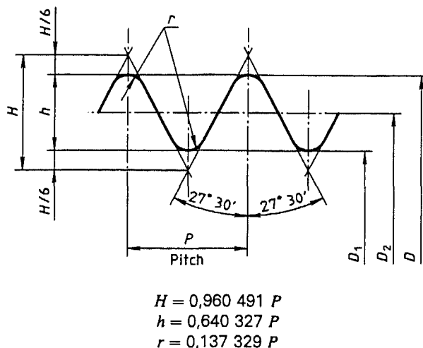
Figure 1 — Parallel thread
