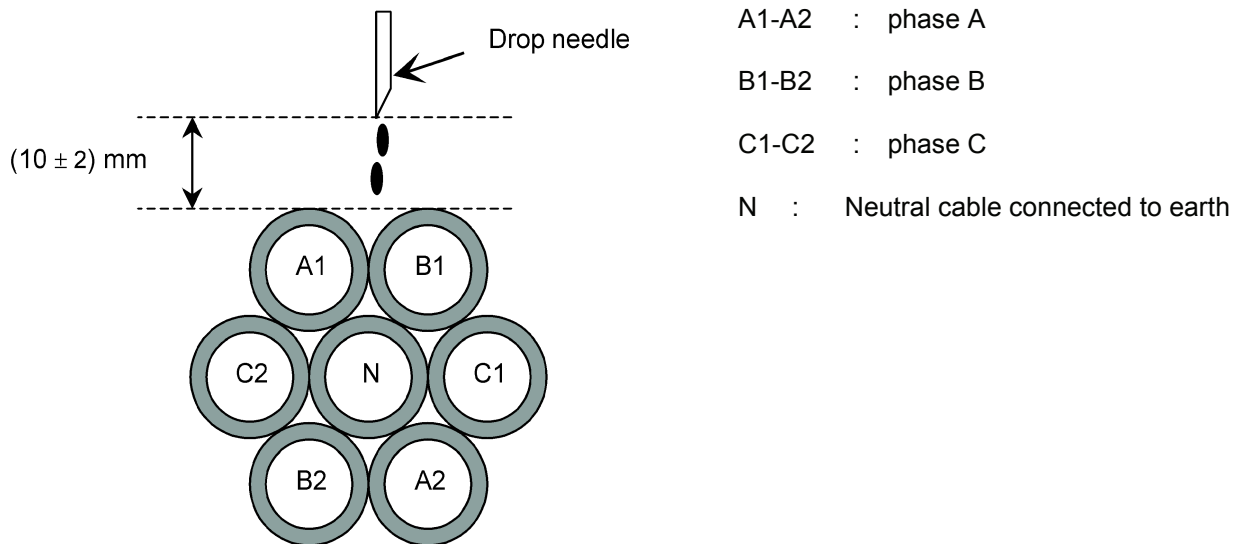
Figure 1 — Specimen configuration
