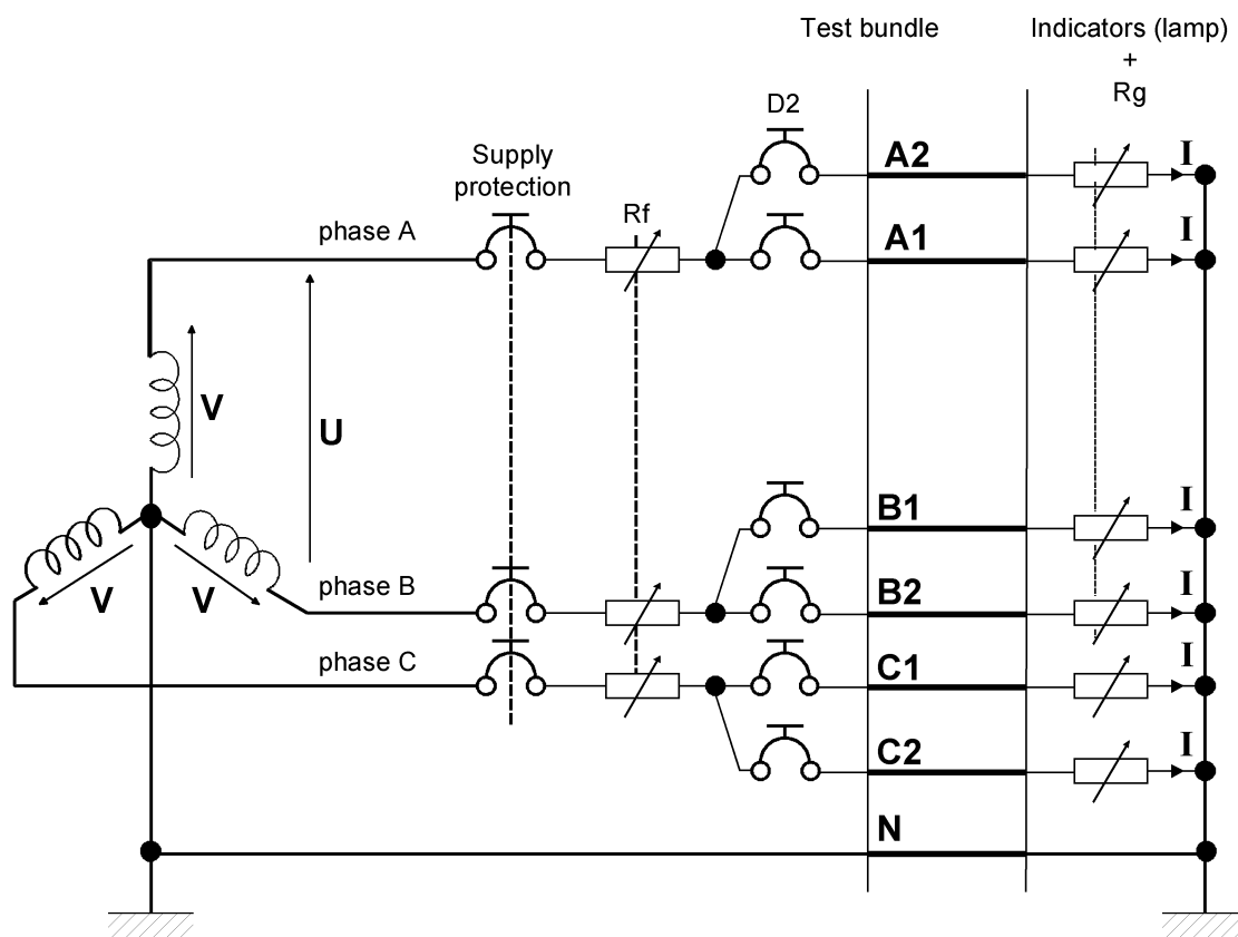
Figure 3 — Test schematic circuit
