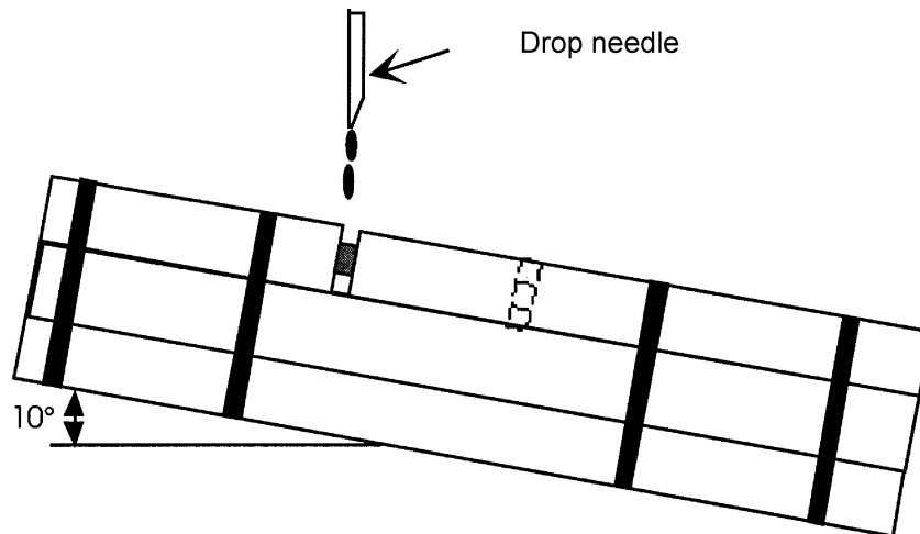
Figure 2 — Test configuration
