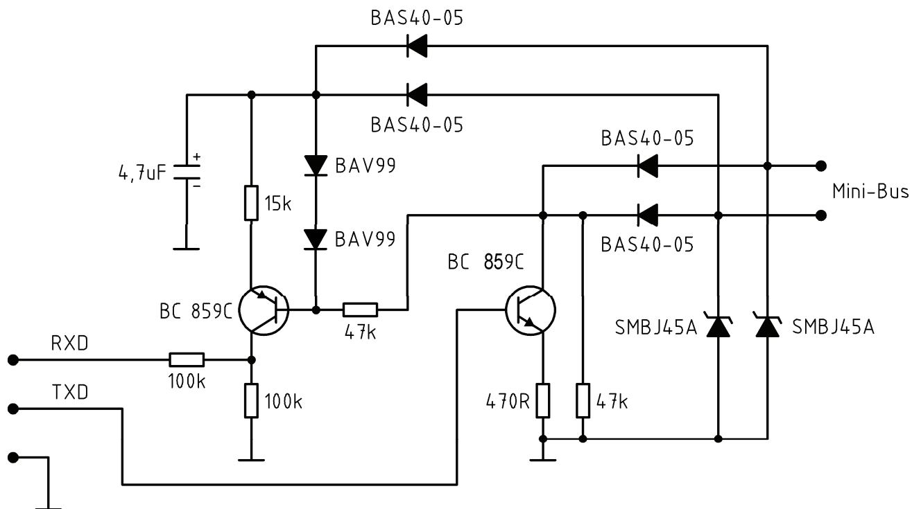
Figure A.1 — Schematic implementation of a meter interface
