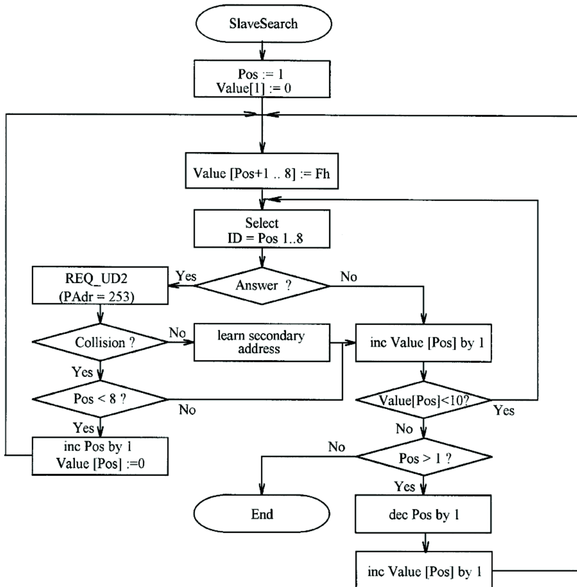
Figure F.2 — Flow Diagram for Slave Search with Wildcards
