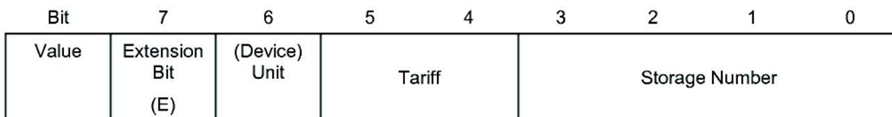
Figure 7 — Coding of the Data Information Field Extension (DIFE)
