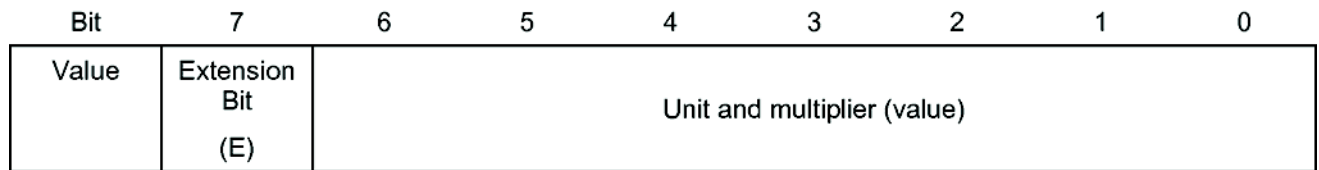
Figure 8 — Coding of the Value Information Field (VIF)
